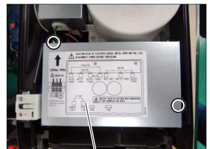
PCB cover
