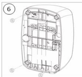
Remove the silent blocks from the back of the unit (x4)
