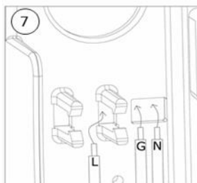
Route the wires through the holes to the back of the unit as shown on the picture
