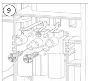
Fix the fast connector to the back of the unit using 2 screws
