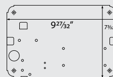
MOUNTING VIEW
