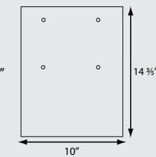
MOUNTING VIEW
