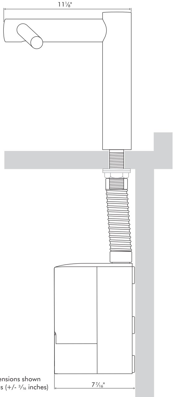
SIDE ELEVATION
